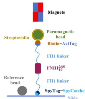
Fibronectin domain with hierarchical symmetry Phys. Rev. Lett. 131 (2023)
