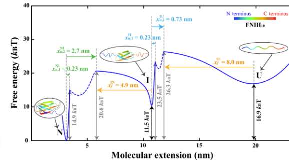
Fibronectin domain with hierarchical symmetry Phys. Rev. Lett. 131 (2023)
