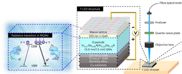
Topology-induced chiral photon emission Nature Electronics 6, (2023)
