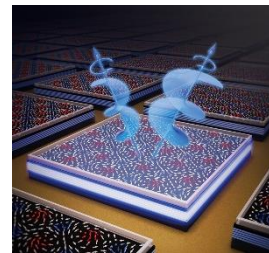
Topology-induced chiral photon emission Nature Electronics 6, (2023)
