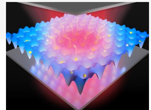
Quantum switch based on microcavity exciton polaritons Nature 591, 61 (2021)
